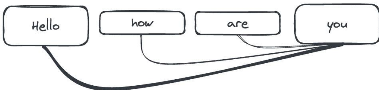
Figure 3.1: Self-attention mechanism
